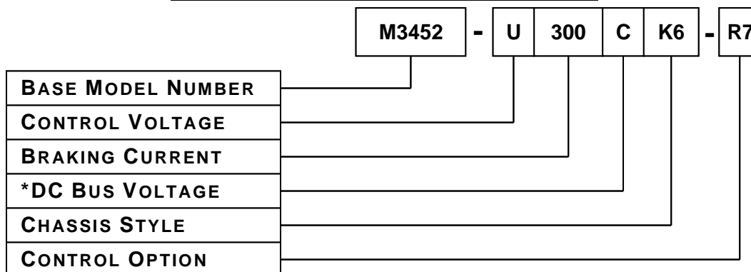
Figure 2-1: M3452 Part Number Breakdown
