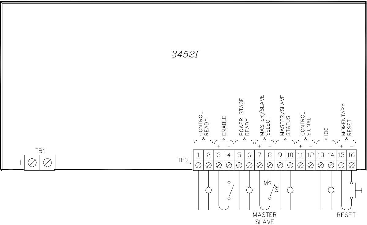
Figure 3-8: I/O Hookup
