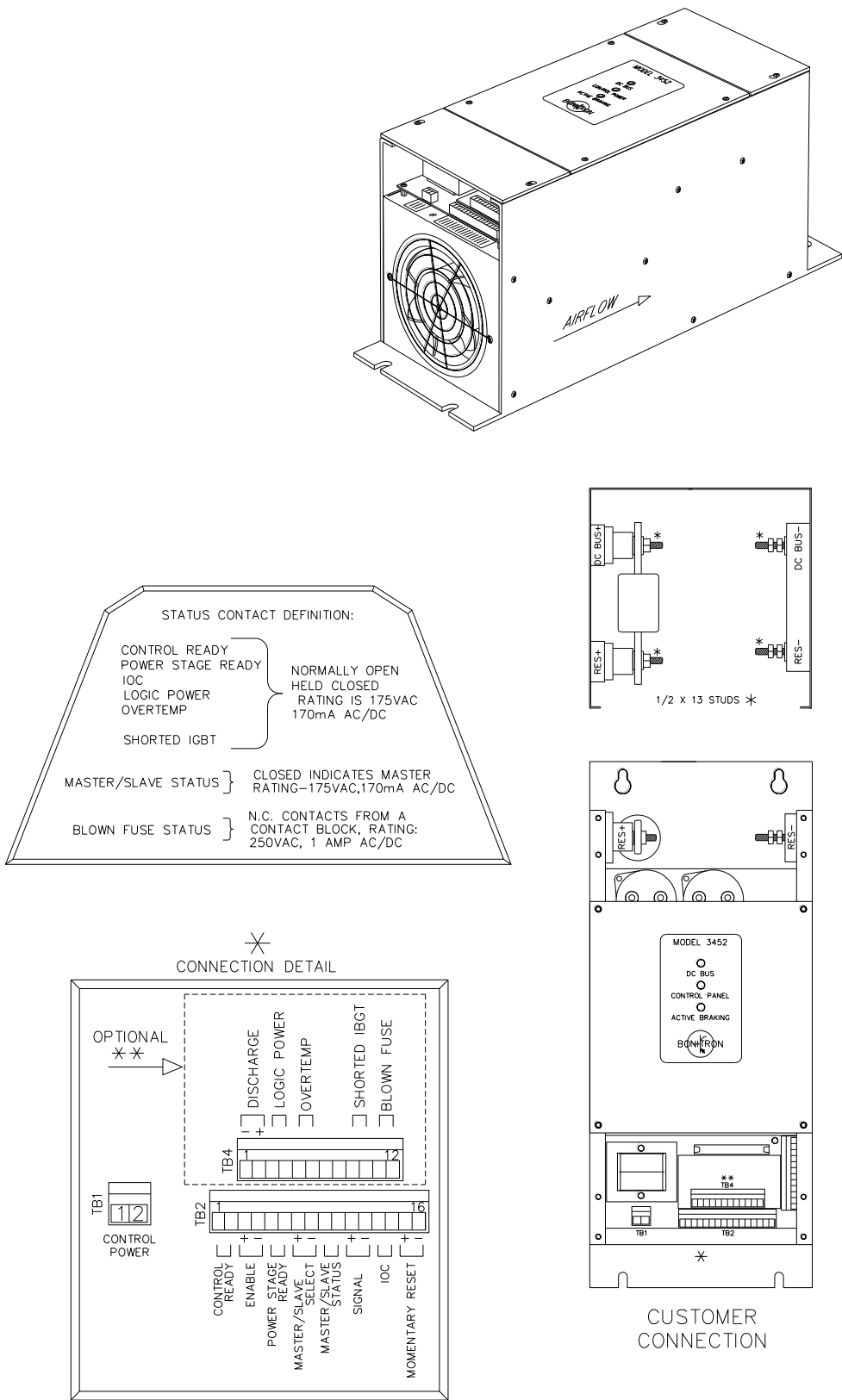
Figure 3-3: Customer Connections in K10 Chassis
