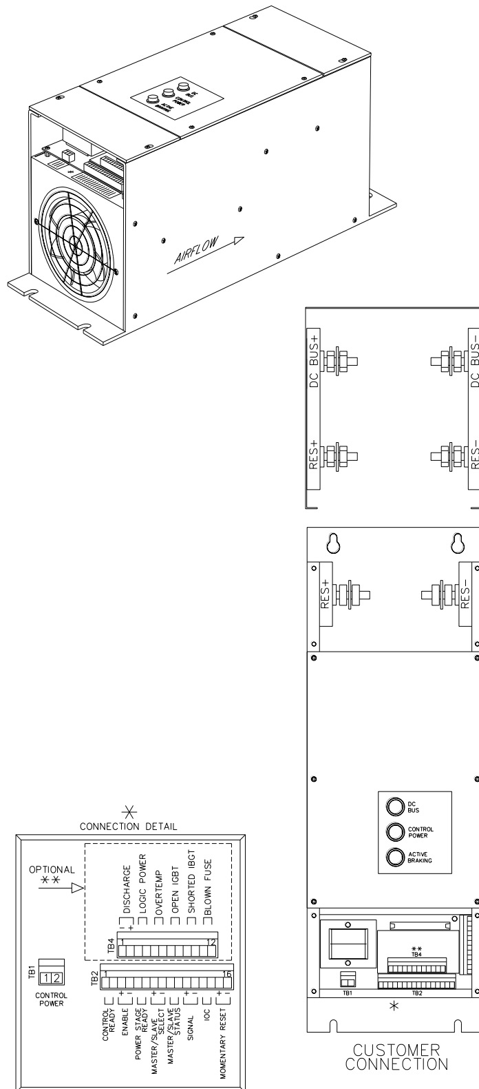
Figure 3-2: Customer Connections in K9 Chassis
