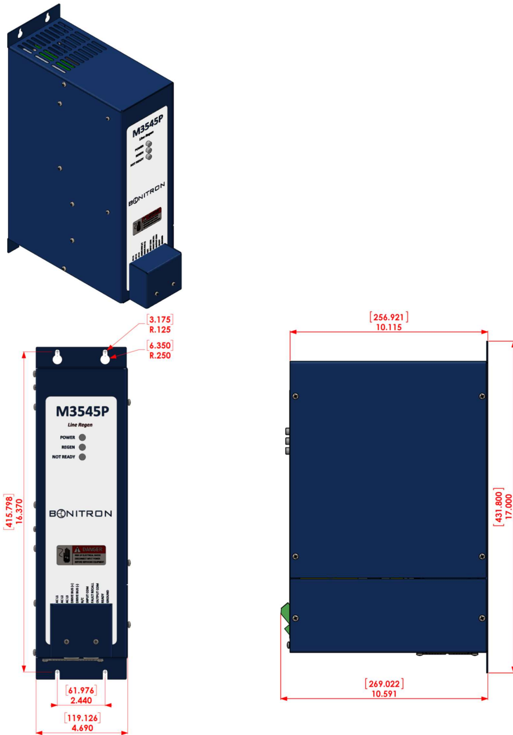
Figure 5-1: M3545P M4 Chassis Dimensional Outline
