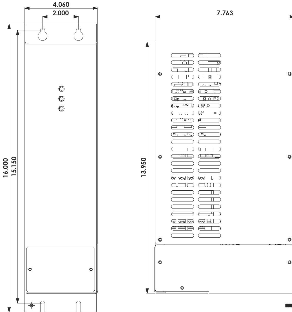
Figure 6 1: M3545P – 6 Amps C4 Chassis Dimensional Outline
