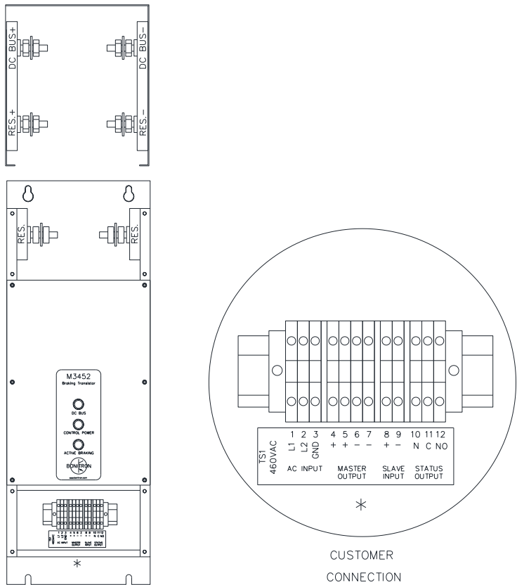
Figure 3-4: Customer Connections in K9 Chassis
