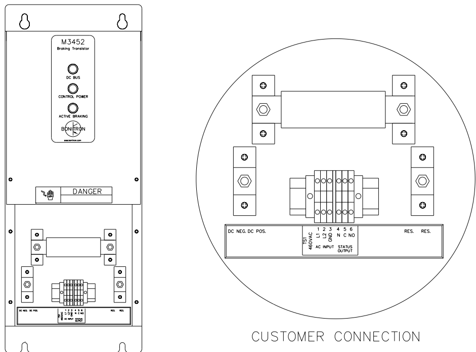
Figure 3-1: Customer Connections in B7 Chassis
