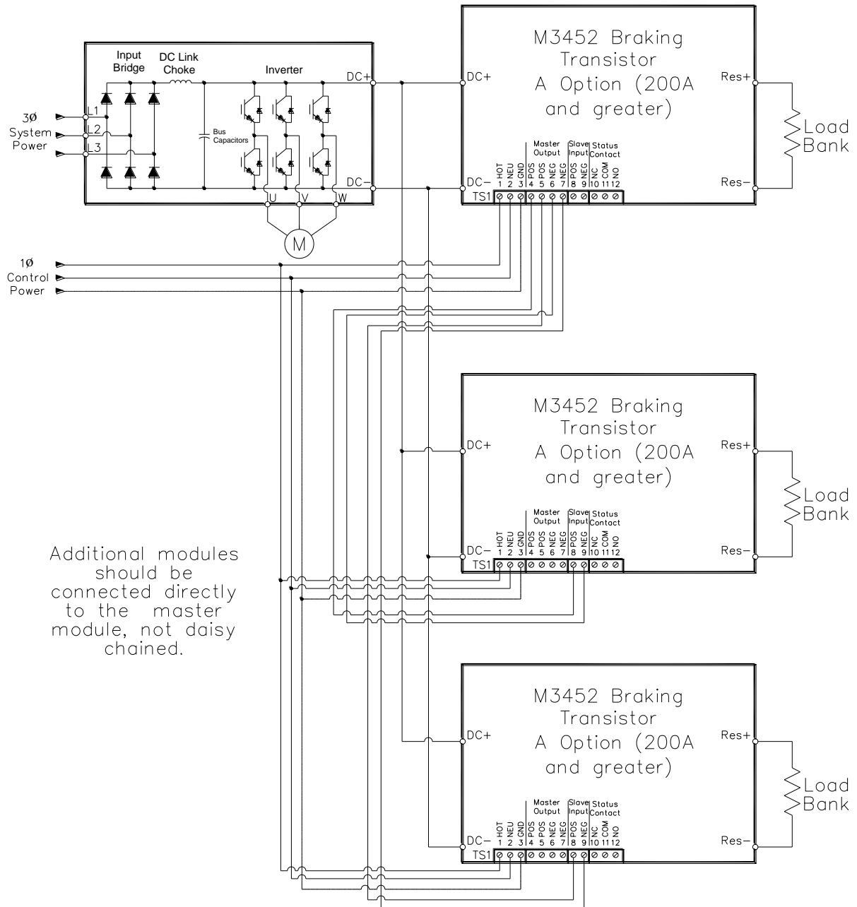
Figure 3-5: Master with Two Slaves Hookup
